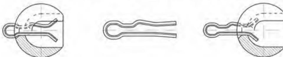
Colter pin "M" acc. to IEC 372
