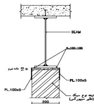
SEC. 1-1 S.C.: 1/10
