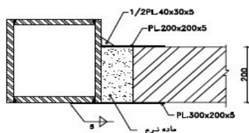
SEC. 2-2 S.C.: 1/10
