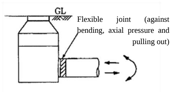
Figure. 6-6 Flexible Joint
