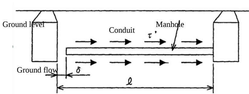
Figure 7-4 the pulling out length of pipe and manhole connection due to liquefaction (for PVC pipe with adhesive joint)
