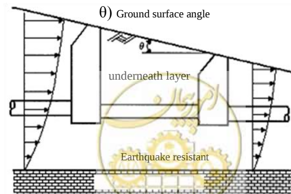
Fig. 6-8 steep ground
