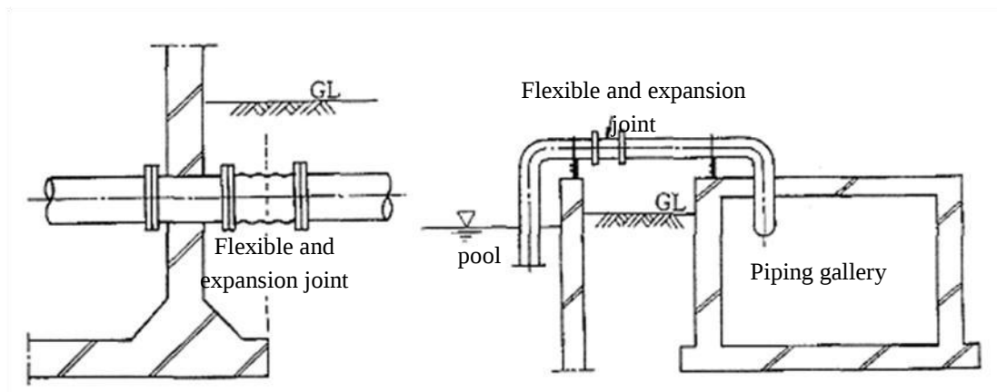
Fig. 5-3 typical flexible joint
