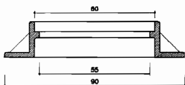
FRAME SECTION
