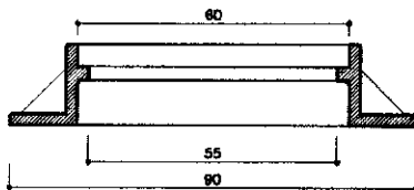
FRAME SECTION
