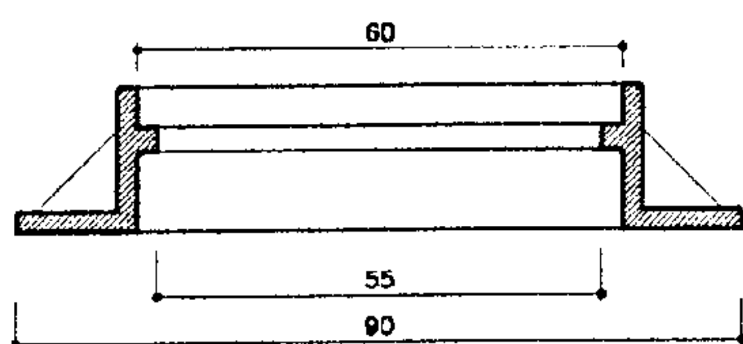
FRAME SECTION
