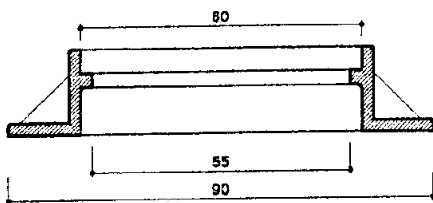
FRAME SECTION
