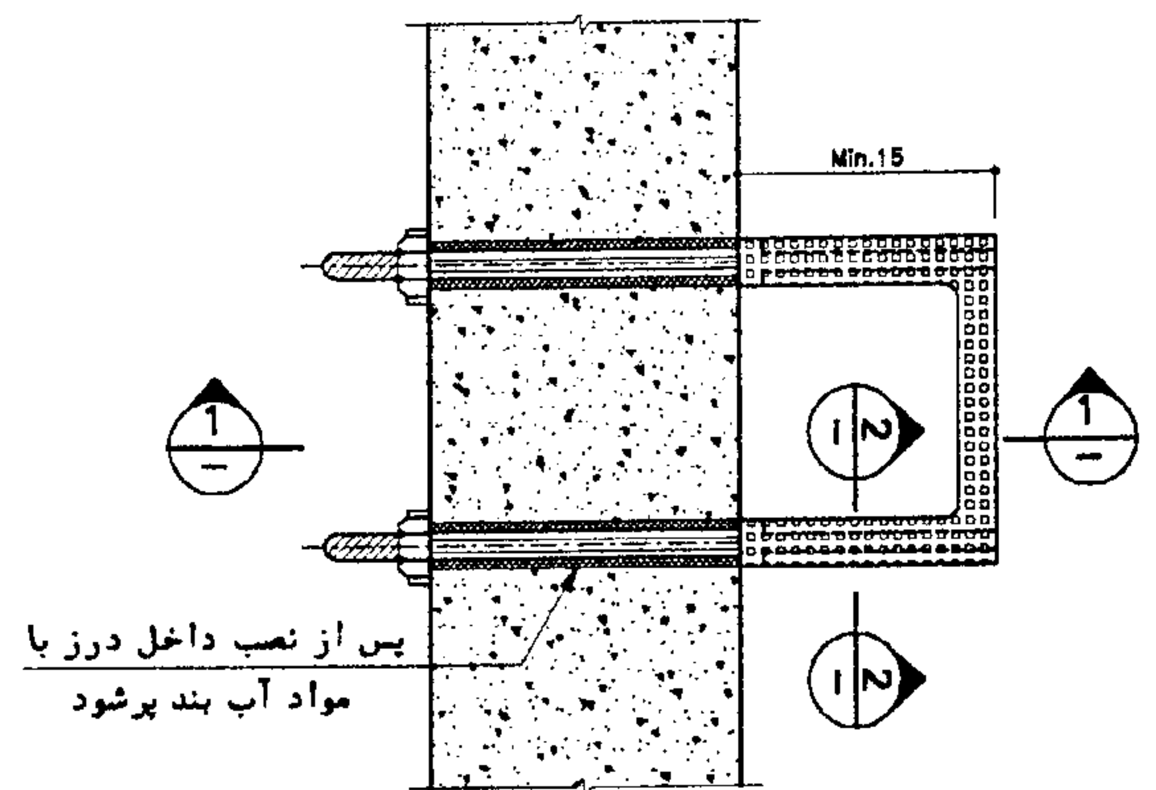
PLAN
