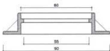
FRAME SECTION
