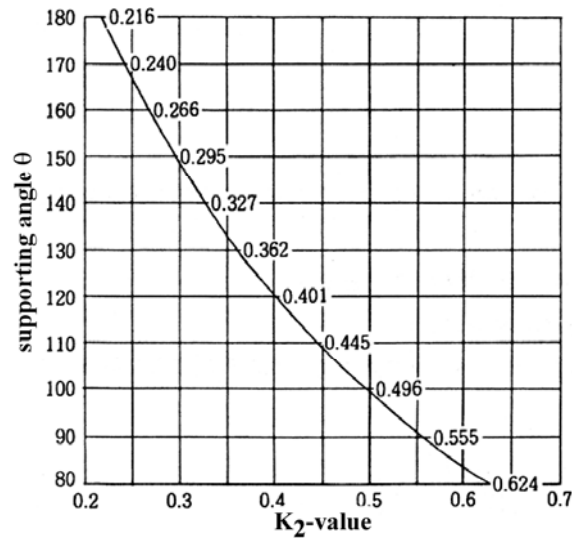
Figure 6.5: Support angle and K 2 value
