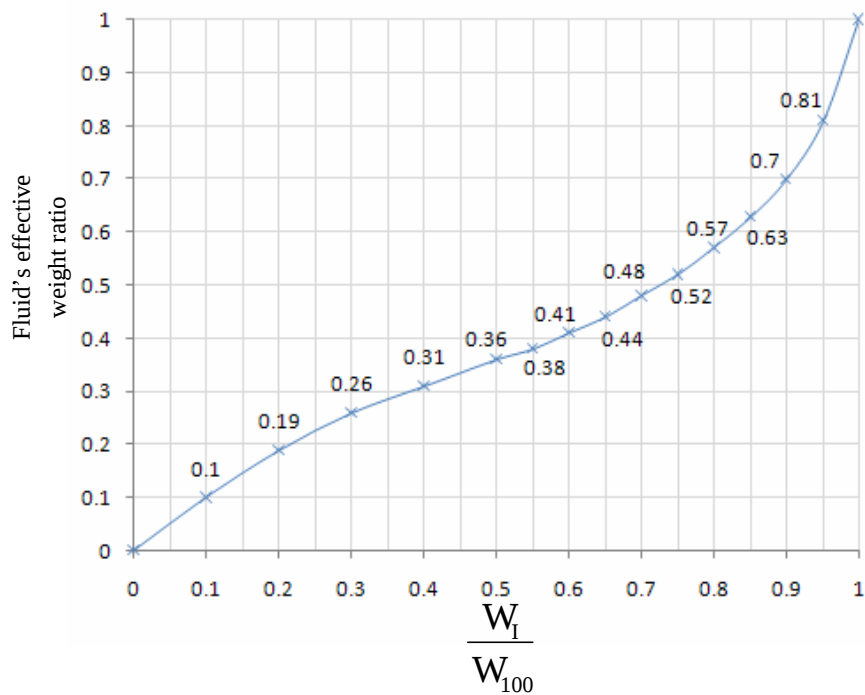
Figure 7.1: Fluid's effective weight ratio
