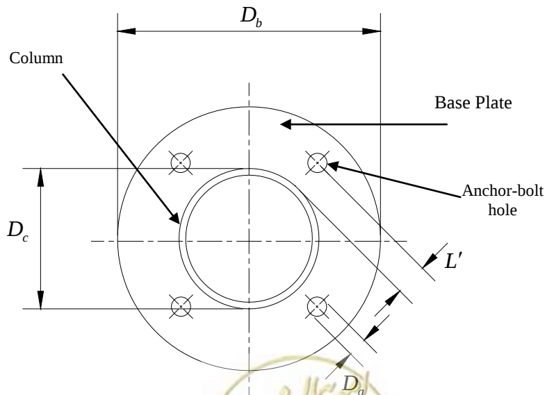
Figure 7.6: Base plate
