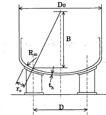
Figure 9.8: Tower with leg support
