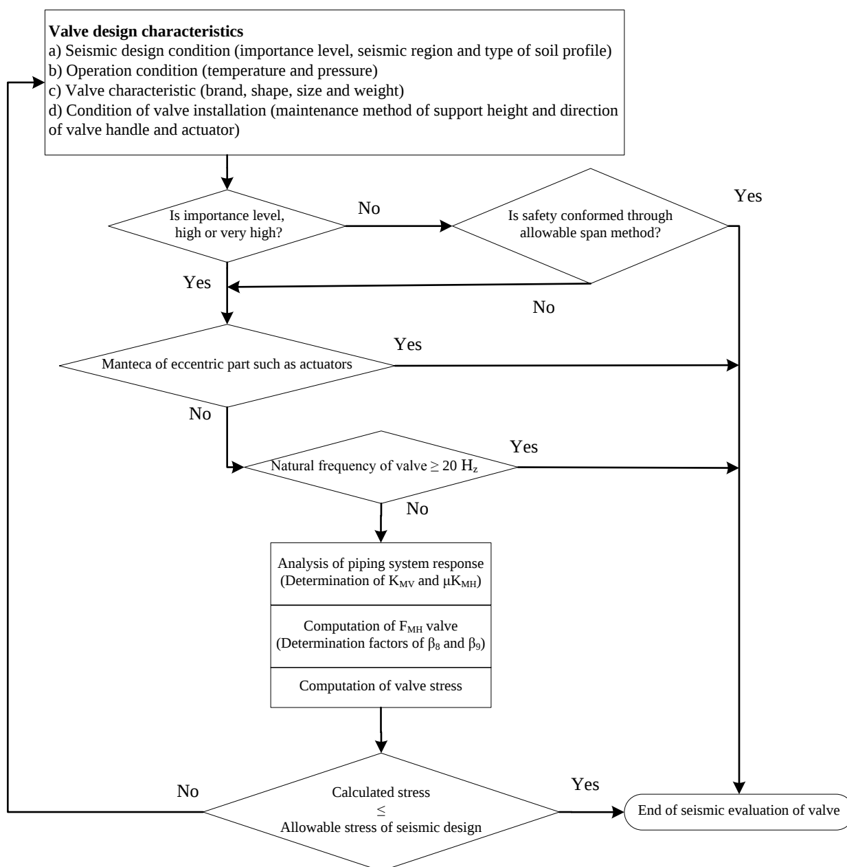
Figure 17-steps of evaluation of valve seismic function
