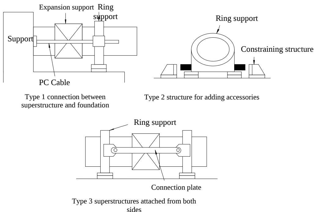
Figure 11.4: Details of constraints and clamps
