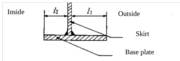
Figure 9.2: Base plate
