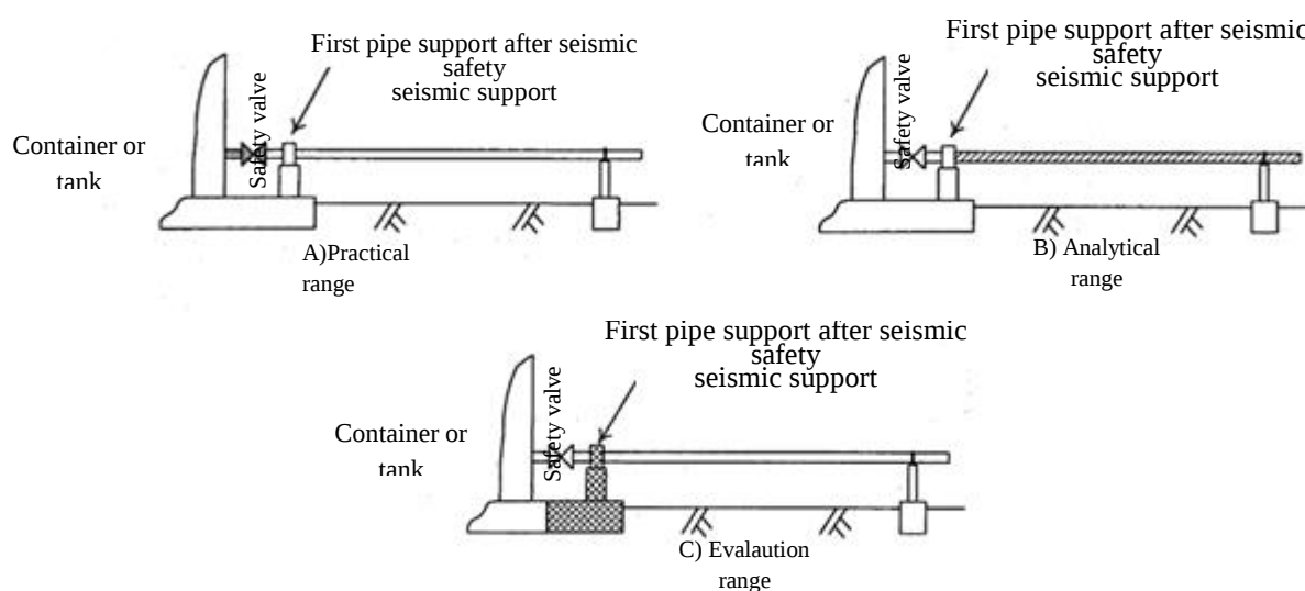
Figure 33-Piping system on common foundation
