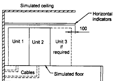
Front elevation
