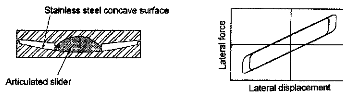
b) Friction pendulum system and the lateral force – displacement relationship
