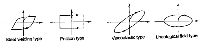
a) Seismic dampers and their idealized lateral force-displacement relationships
