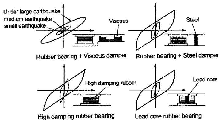
a) Isolation bearings and their lateral force – displacement relationships
