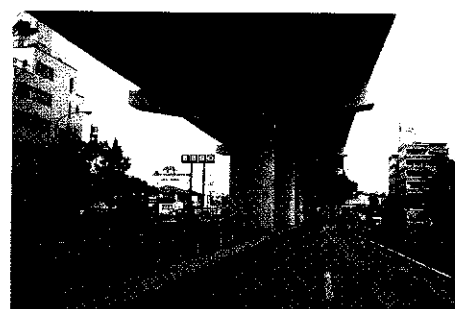
b) Hybrid piers (RC column and steel beam)
