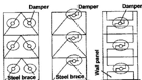
b) Installation example of seismic dampers
