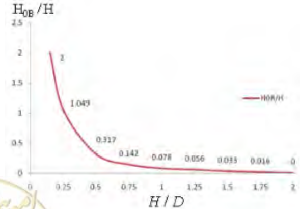
figure 6-5: The relationship between \frac{H}{D} & \frac{H_{0B}}{H}
