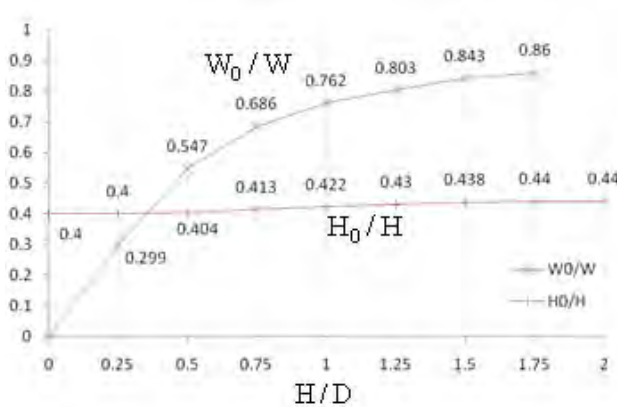
figure 6-2: The relationship between \frac{H}{D} & \frac{W_0}{W} and \frac{H}{D} & \frac{H_0}{H}
