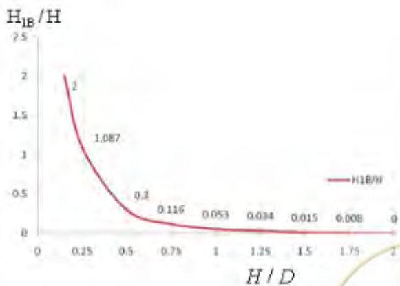
figure 6-4: The relationship between \frac{H}{D} & \frac{H_{1B}}{H}
