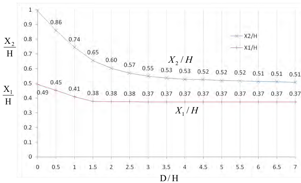
Figure (7-5): Effective weight / height of center of gravity ratio
