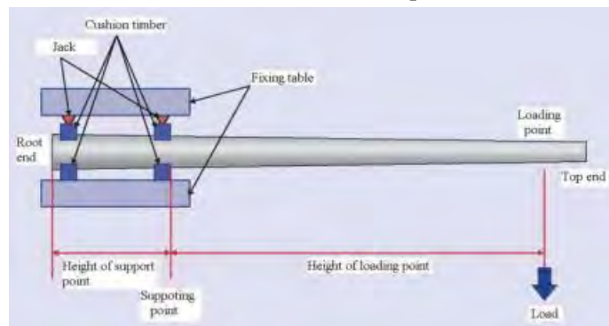
Fig. 10-15: Calculation of conic angle of the pole (left)
